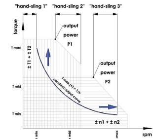
Picture 6: Telescoping L-output with two drives and three "hand-slings" (Source: Kabel.Consult.Ing)
