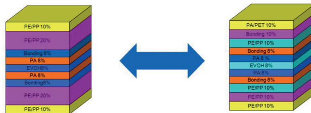
Comparison between 9- and 11-layer blown film
