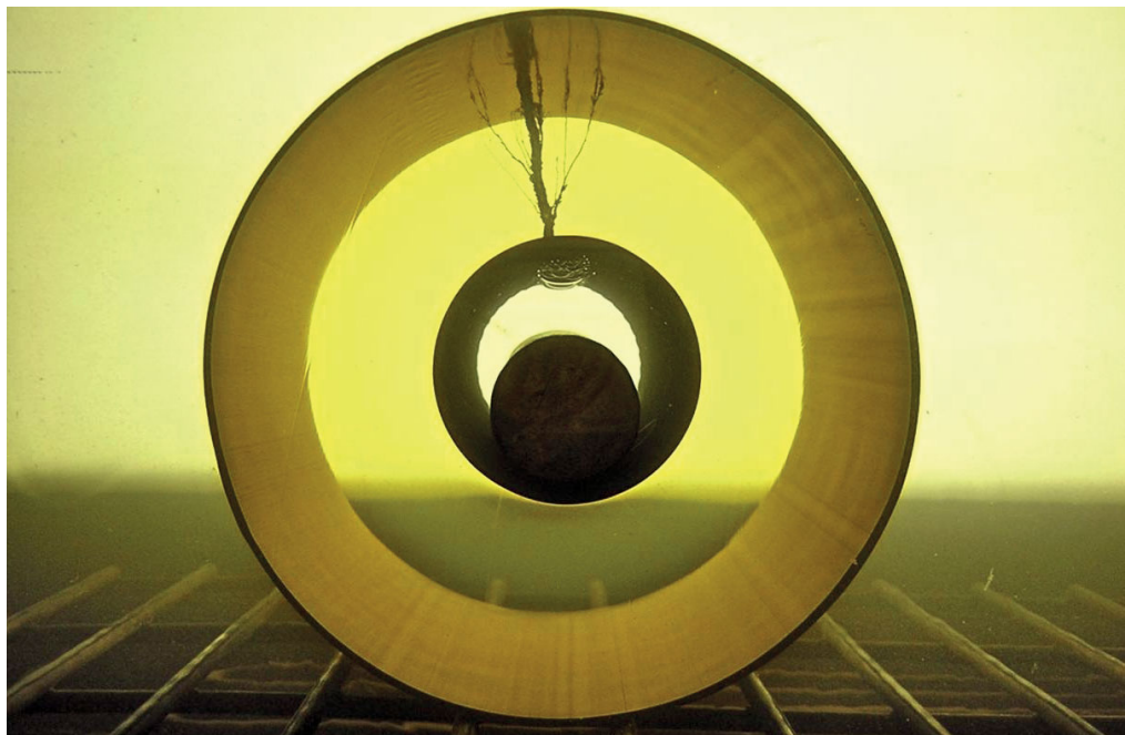
Cross section of an extra-high voltage cable with discharge
